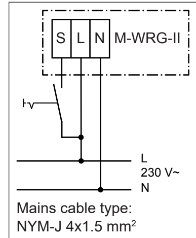
Fig. 48: Connection diagram for external control input
